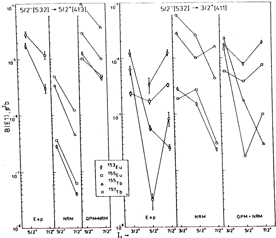
Fig.4. The reduced probabilities of E1 transitions between the members of the 5/2^- [532] band and the 5/2^+ [413] and 3/2^+ [411] bands in ^{153,155}\text{Eu} and ^{155,157}\text{Tb} calculated within the NRM and the present model labeled as the QPM + NRM
