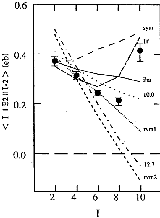
Fig. 1. The experimental and calculated values [21] of the I_{\gamma} \rightarrow (I-2)_{gr} matrix elements in ^{166}\text{Er} . The calculations were performed within the symmetric rotor model (sym), the asymmetric rotor model [32] ( \gamma = 10^\circ and 12.7^\circ , respectively), the rotation-vibration model [33] (rvm1 and rvm2), the IBA-1 model [34] (iba) and a two-rotor model [22] (tr). The adiabatic behavior corresponds to the results of the symmetric rotor model
