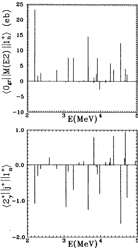
Fig.2. The calculated reduced E2 matrix elements \langle 0^+_{gr} || M(E2) || 1^+_n \rangle and Coriolis coupling matrix elements \langle 2^+_{\gamma} || j^+ || 1^+_n \rangle in ^{166}\text{Er}
