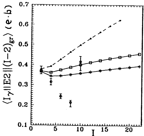
Fig.3. The reduced E2 matrix elements for the I_{\gamma} \rightarrow (I-2)_{gr} transitions in ^{166}\text{Er} : o — experimental data, • — adiabatic calculations, — nonadiabatic calculations with e_{\text{eff}} = 0.02 , * — nonadiabatic calculations with e_{\text{eff}} = 0.3 (see the text)
