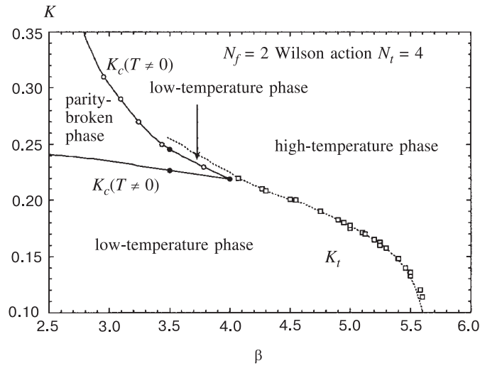
Fig. 12. The finite temperature phase diagram in the (\beta, \kappa) plane for standard Wilson fermions [51]
