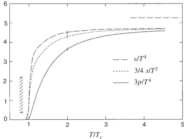
Fig. 15. The extrapolated continuum limit of energy density, entropy density and pressure in the pure glue theory [2]. The dashed horizontal line shows the ideal gas limit. The hatched vertical band indicates the size of the discontinuity in \epsilon/T^4 (latent heat) at T_c [62]
