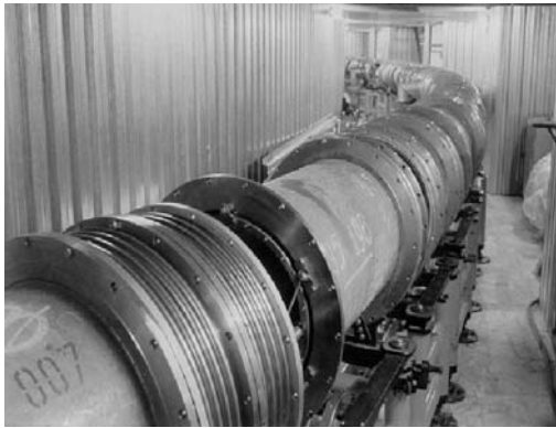
The Nuclotron — superconducting synchrotron for heavy ions up to 6 GeV/nucleon — has been operating since 1993
