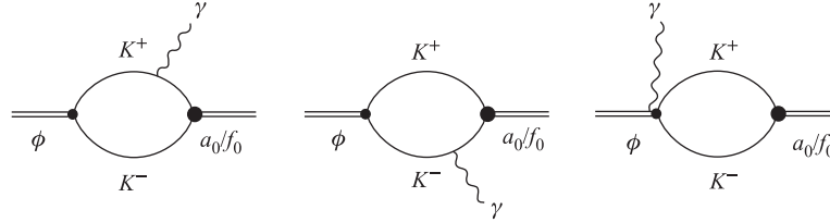
Fig. 3. The K^+K^- loop model
