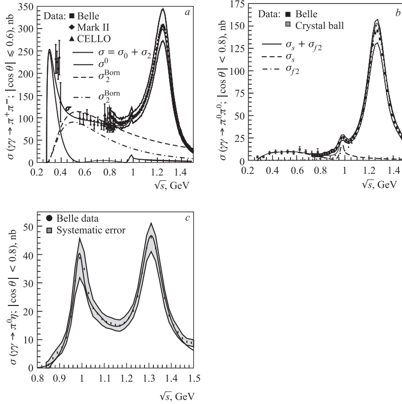
Fig. 5. Descriptions of the Belle data on \gamma\gamma \rightarrow \pi^+\pi^- (a), \gamma\gamma \rightarrow \pi^0\pi^0 (b), and \gamma\gamma \rightarrow \pi^0\eta (c)
