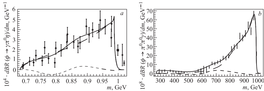
Fig. 4. The plot a(b) shows the fit to the KLOE data for the \pi^0\eta ( \pi^0\pi^0 ) mass spectrum in the \phi \rightarrow \gamma\pi^0\eta ( \phi \rightarrow \gamma\pi^0\pi^0 ) decay caused by the a_0(980) ( \sigma(600) + f_0(980) ) production through the K^+K^- loop mechanism
