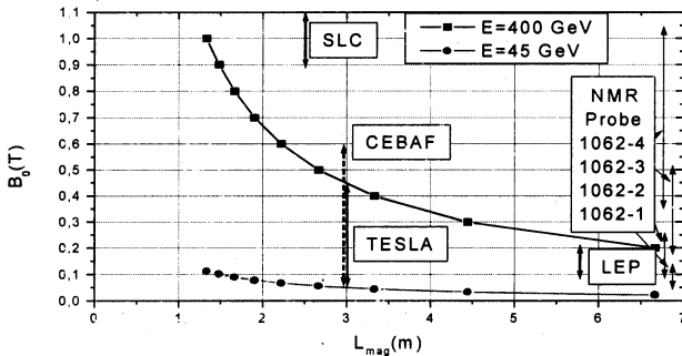
Fig.2. B_0=f(L_{\text{mag}}) relations for the TESLA spectrometer magnet
