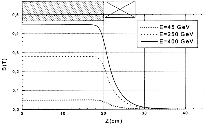
Fig.17. Magnetic field distribution in the Z direction of the spectrometer magnet
