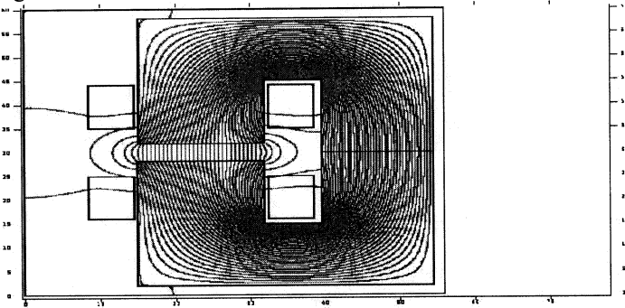
Fig.8. POISSON SUPERFISH model 1 showing magnetic flux lines
