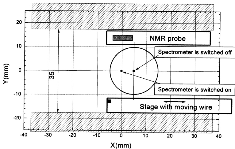
Fig.6. Cross-sectional view of the spectrometer magnet pole gap
