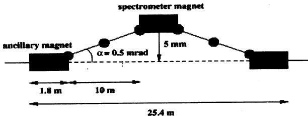
Fig.1. TESLA magnetic spectrometer
