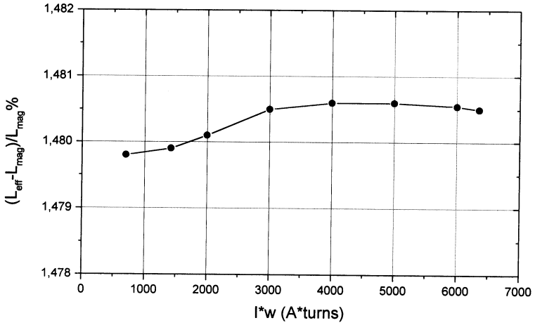
Fig.18. Normalized effective length of the spectrometer magnet
