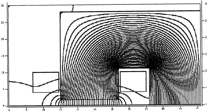
Fig.8. POISSON SUPERFISH model 1 showing magnetic flux lines
