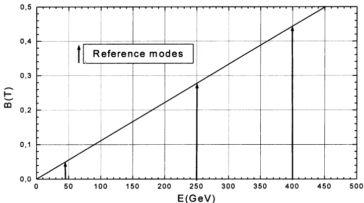
Fig.5. Working line of the TESLA spectrometer magnet
