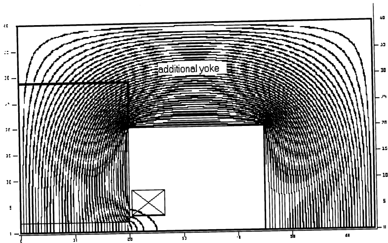
Fig.10. POISSON SUPERFISH model 3 showing magnetic flux lines
