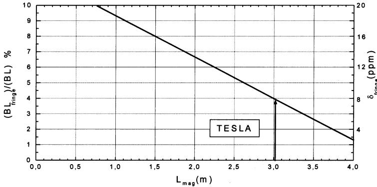
Fig.4. Fraction of the fringe field integral and the relative accuracy of the fringe field measurement by the Hall probe
