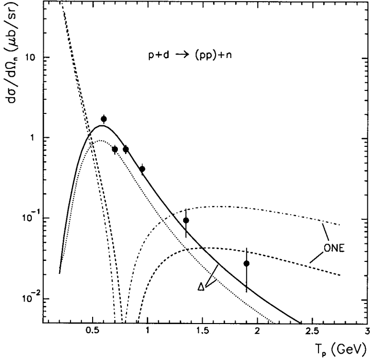
Figure 3: Contributions of the considered reaction mechanisms to the cms differential cross section of the reaction p + d \rightarrow (pp) + n at neutron scattering angle \theta_n^* = 172 - 180^\circ and relative energies E_{pp} = 0 - 3 MeV of the two forward protons. Results are shown for the Paris (ONE - dash-dotted line, \Delta - dotted line) and CD Bonn (ONE - dashed line, \Delta - solid line) NN potentials. Data are from Ref. [12].
