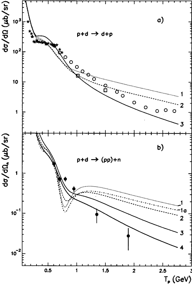
Figure 2: Cms differential cross sections of the reaction pd \rightarrow dp at the proton scattering angle \theta_p^* = 180^\circ (a) and of the reaction p + d \rightarrow (pp) + n for neutron scattering angles \theta_n^* = 172 - 180^\circ and relative energies E_{pp} = 0 - 3 MeV of the two forward protons (b) as a function of the beam energy T_p . Calculations are performed on the basis of the ONE+SS+ \Delta model described in the text without (lines 1–3) and with distortions included (4) for the RSC (1), Paris (2) and the CD Bonn (3,4) potentials. The curve 1a shows the result for the RSC potential with Coulomb effects included. Curve 4 is the result for the CD Bonn potential taking into account distortions for the ONE mechanism and also Coulomb effects (by the suppression factor of 20%, cf. text). Data for pd \rightarrow (pp)n are from Ref. [12], and for pd \rightarrow dp from [21, 22, 23].
