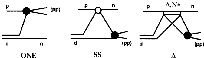
Figure 1: Mechanisms of the breakup reaction pd \rightarrow (pp)n . The same mechanisms are used for the reaction pd \rightarrow dp .
