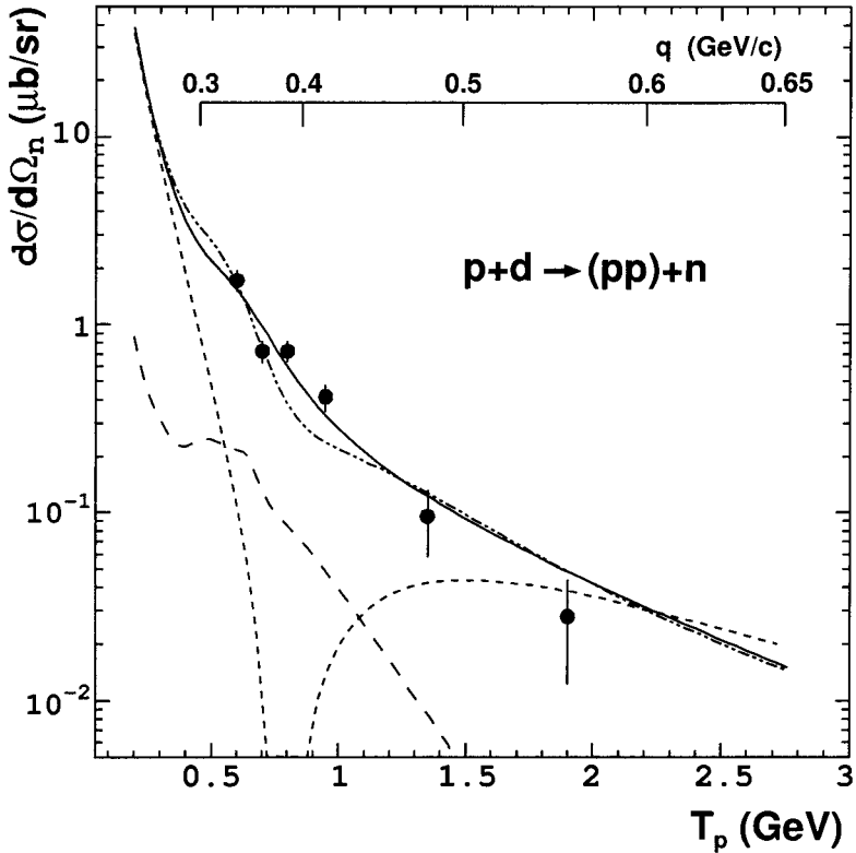
Figure 4: The same as in Fig. 3, but using the CD Bonn NN potential only. ONE – short-dashed line; SS – long-dashed line; coherent sum of ONE+ \Delta with Coulomb effects included – solid line; ONE+SS+ \Delta with Coulomb effects included – dashed-double dotted line. In the latter two cases distortions in the ONE contribution are also included. The upper scale shows the internal momentum of the nucleons in the deuteron for the ONE, cf. Eq. (2).
