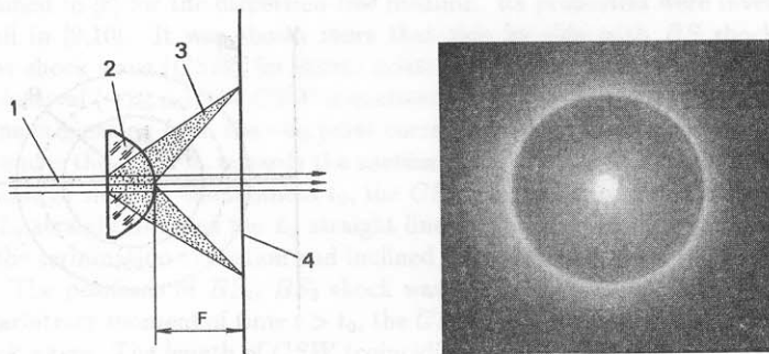
Figure 2: Left: The scheme of experiment with the lense radiator; 1 is the proton beam, 2 is the lense radiator, 3 is the focused VC radiation, 4 is the plane photofilm placed perpendicularly to the motion axis, F is the focal distance for paraxial rays; Right: the black-white photoprint from the photofilm shown on the left.
