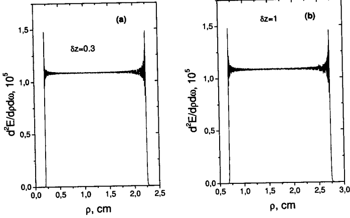
Figure 8: Exact theoretical radiation intensities in the \delta z = 0.3\text{cm} and \delta z = 1\text{cm} planes.
