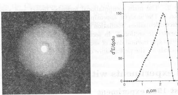
Figure 4: Left: The black-white photoprint from the photofilm shown in Fig. 3; Right: The photometric curve corresponding to the left part. One observes the increment of the radiation intensity at \rho \approx 2.25\text{cm} which corresponds to the Cherenkov ray emitted from the point where the proton beam enters the radiator.
