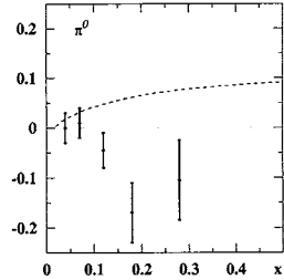
A_{UT}^{\sin(\phi+\phi_h)}(x) vs. HERMES preliminary
