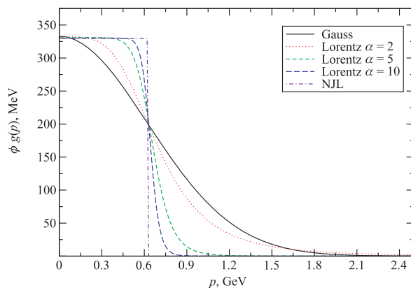
Fig. 2. The gap functions of light quarks for different form factor models. The present parameter set is from Table 2
