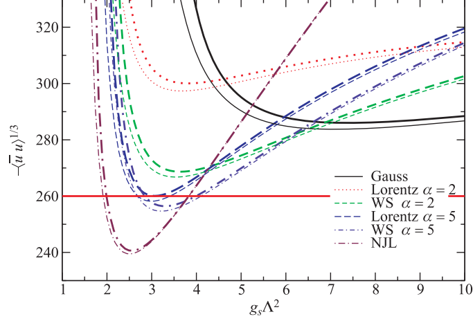
Fig. 1. The dependence of the chiral condensate -\langle\bar{u}u\rangle^{1/3} on the choice of the coupling constant in the chiral limit (thick lines) and for finite current mass of the light quark m_0 \simeq 0.01 \Lambda (thin lines) for different form factor models. The plot demonstrates that not for all cases the phenomenological constraint for the value of the condensate from QCD sum rules [21] with an upper limit at 260 MeV can be fulfilled
