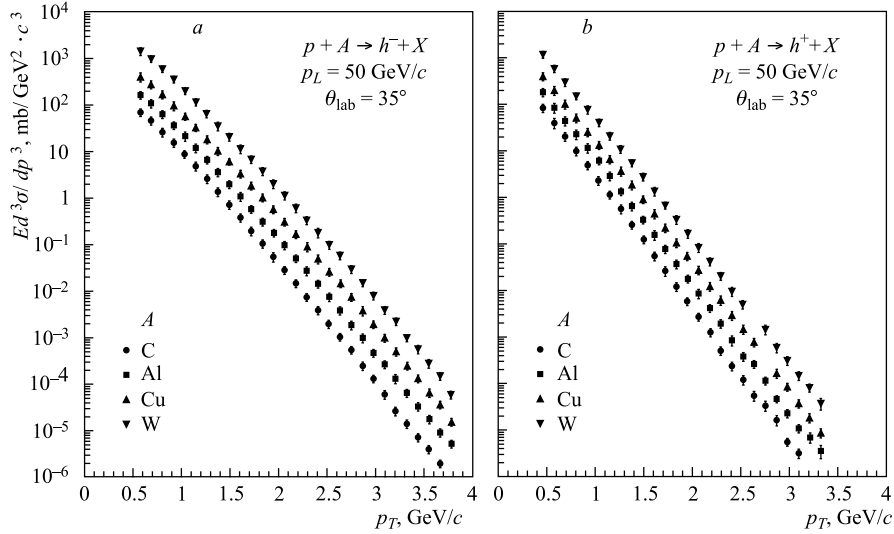
Fig. 1. Spectra of h^- (a) and h^+ (b) hadrons produced in p + A collisions at incident proton momentum p_L = 50 GeV/ c and angle \theta_{\text{lab}} = 35^\circ as a function of transverse momentum p_T . The experimental data are taken from [30]
