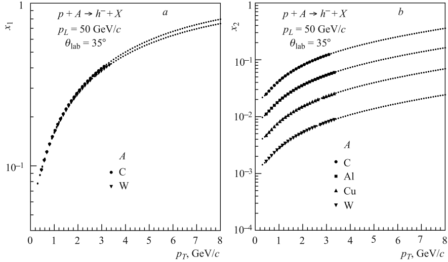
Fig. 4. Dependence of the fractions x_1 (a) and x_2 (b) on momentum p_T of h^- hadrons produced in p + A collisions at p_L = 50 GeV/c and \theta_{\text{lab}} = 35^\circ
