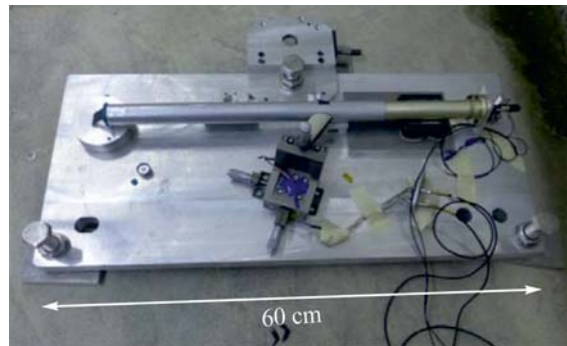
Fig. 3. Precision Laser Incliner location in the Transfer Tunnel#1
