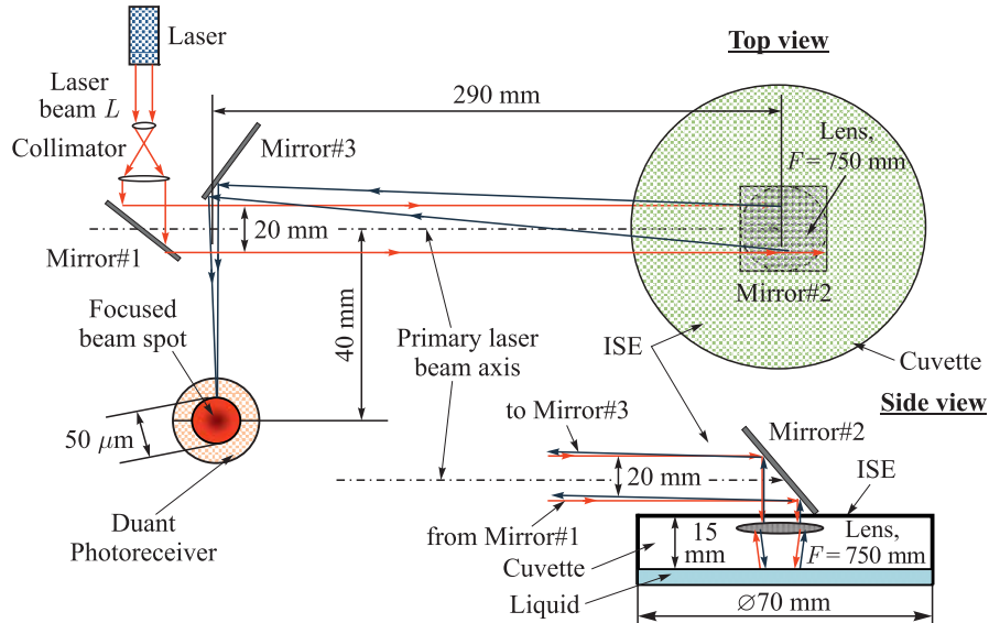
Fig. 1. The principal scheme of the Precision Laser Inclinometer
