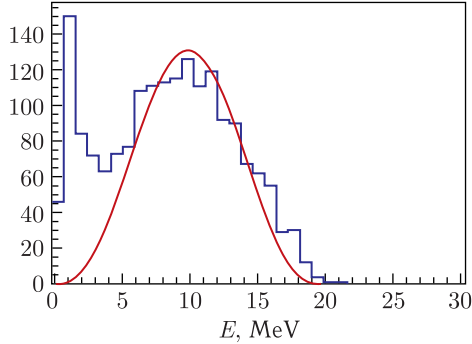
Fig. 4. Experimental (histogram) and model (solid line) energy spectra of one of two \gamma quanta from reaction (2) (exposure III)
