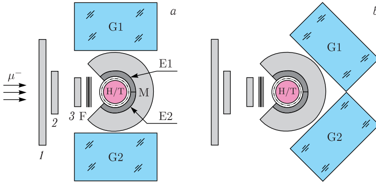
Fig. 1. Scheme of the experiment: a ) for exposures I, II, IV; b ) for exposure III; 1–3 — muon beam counters, F — copper muon moderator, H/T — target, E1, E2 — electron detectors, M — muon detector, G1, G2 — \gamma -ray detectors
